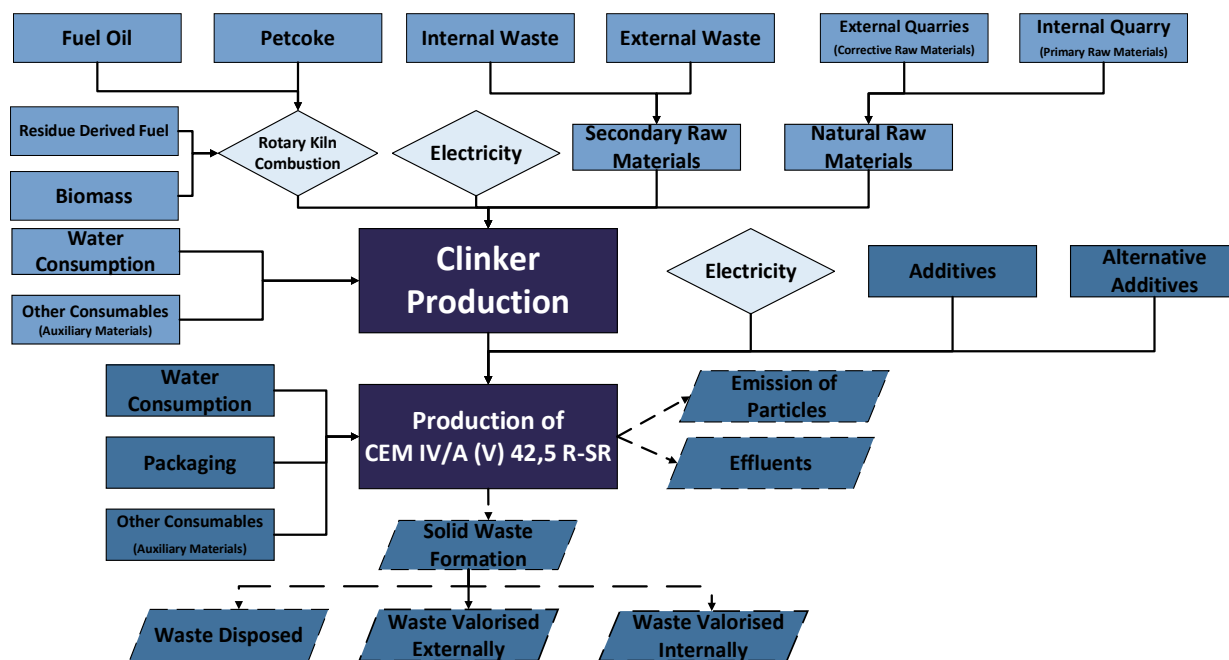
Figure 1: Simplified flowchart for CEM IV/A (V) 42,5 R-SR cement production inventory.
