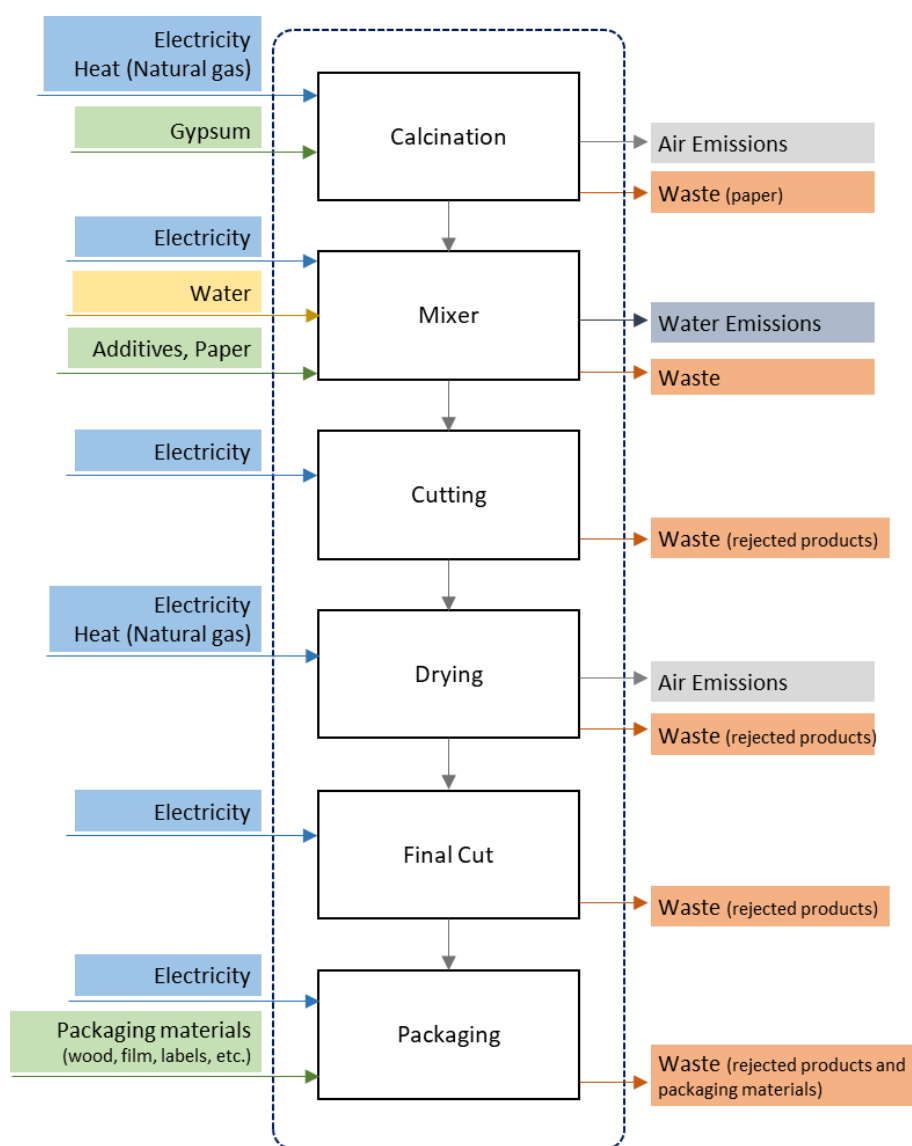
Figure 2: Production process of Standard Gypsum Plasterboard.
