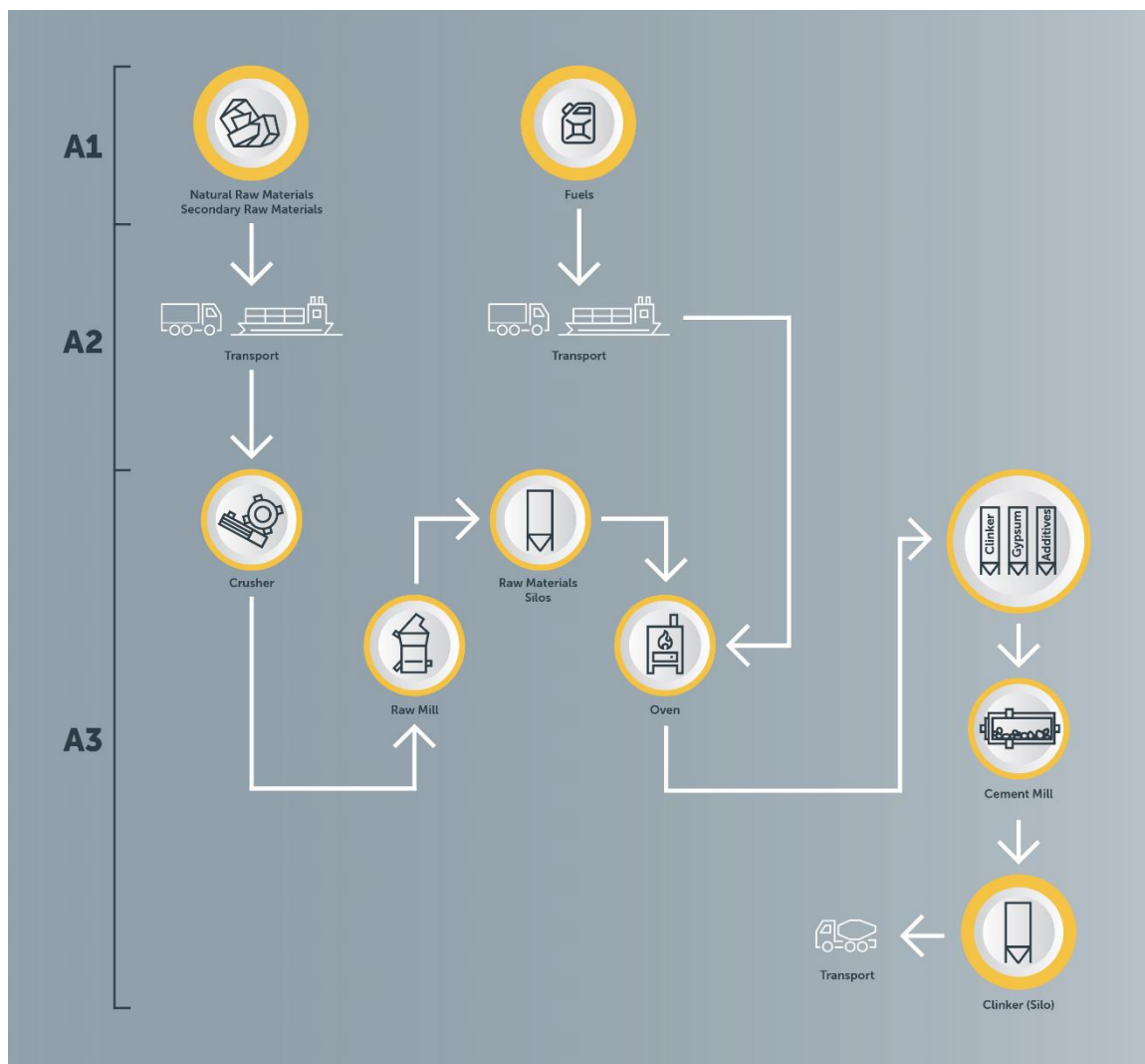
Figure 1: Flowchart of the manufacturing process of CEM I 52.5R Portland cement
