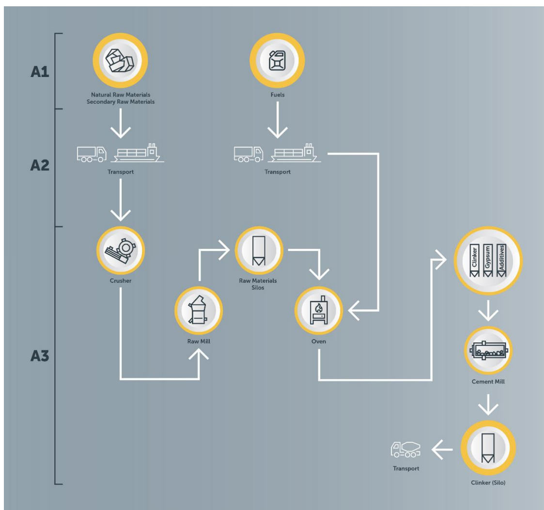
Figure 1: Flowchart of the Portland cement manufacturing process
