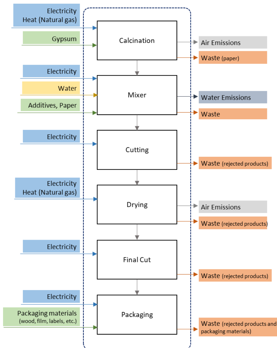
Figure 2: Production process of Fire Resistant Gypsum Plasterboard.
