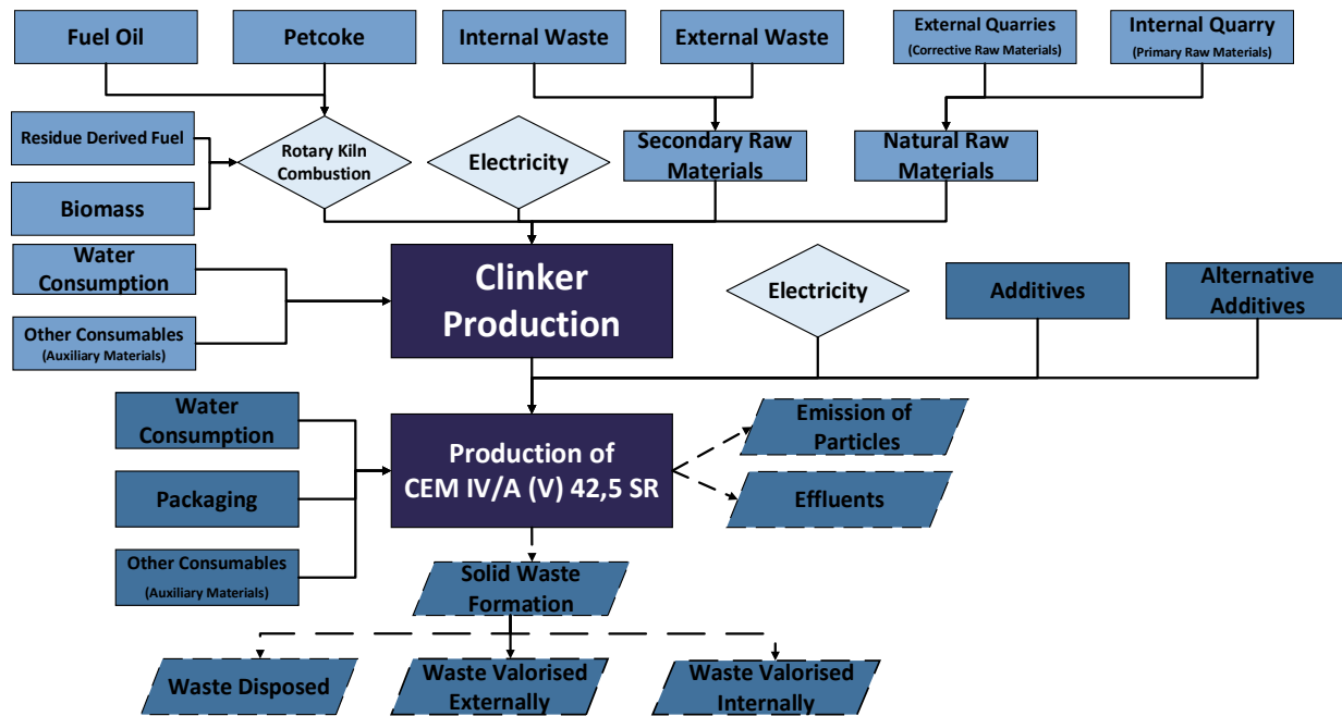
Figure 1: Simplified flowchart for CEM IV/A (V) 42,5 SR cement production inventory.
