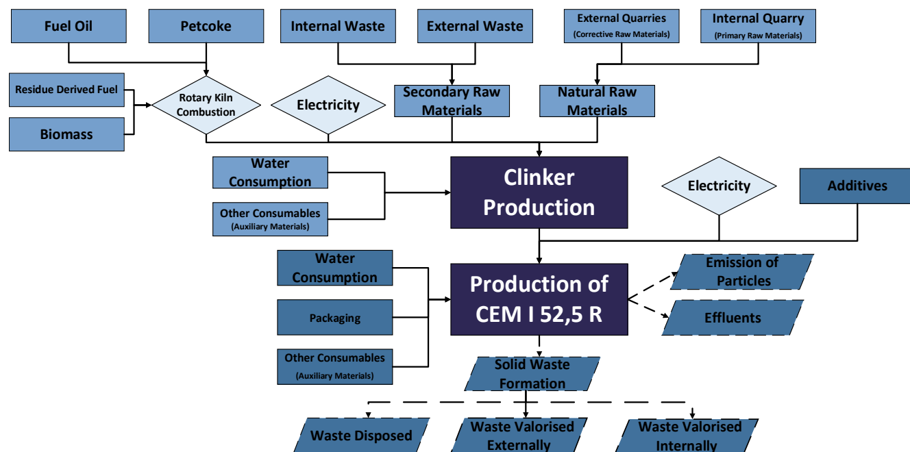
Figure 1: Simplified flowchart for CEM I 52,5 R cement production inventory.
