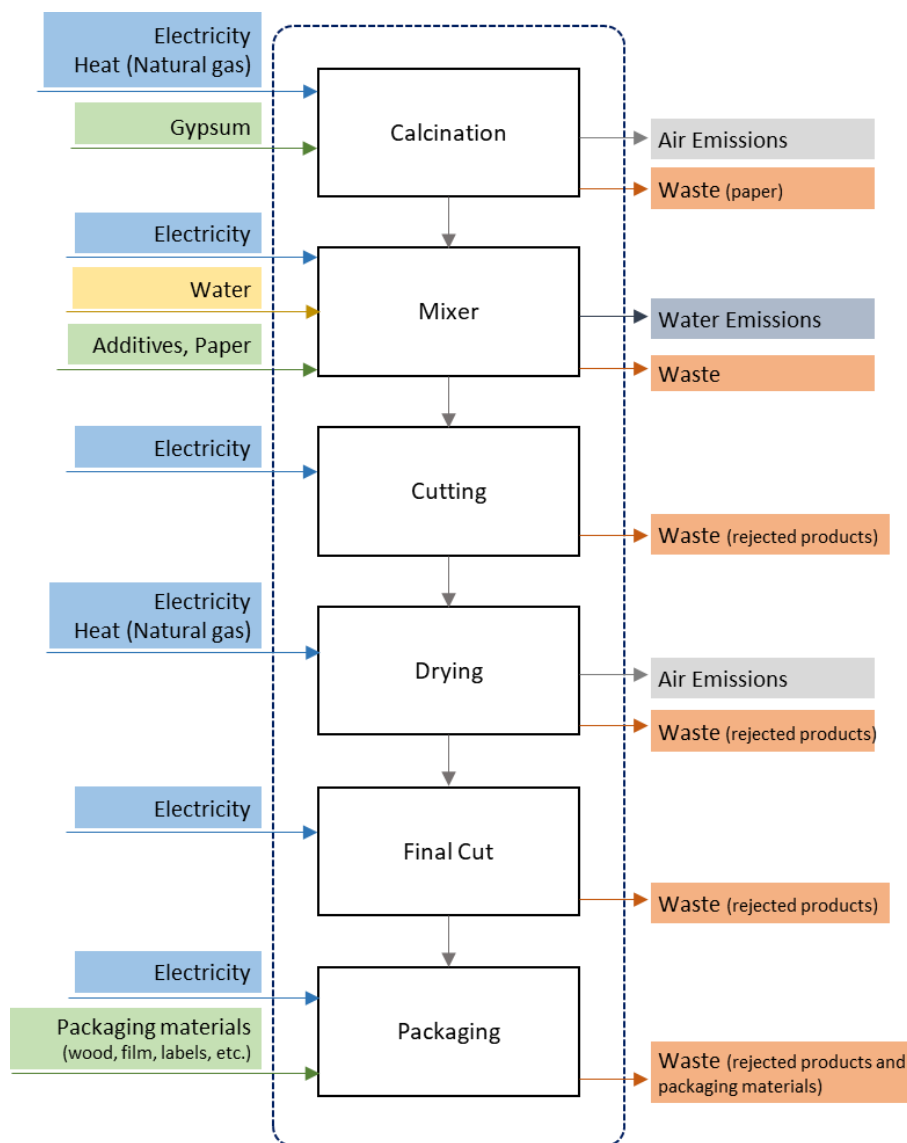
Figure 2: Production process of Gold Gypsum Plasterboard.
