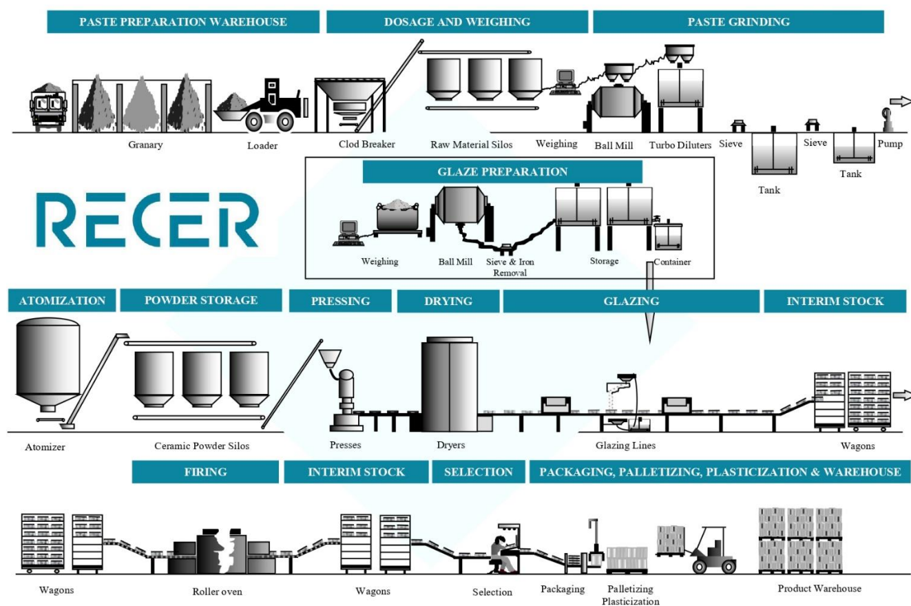
Figure 1 - Production process
